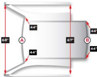
TRADITIONAL ROOF
