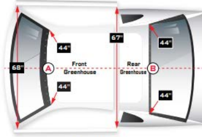
GREENHOUSE
